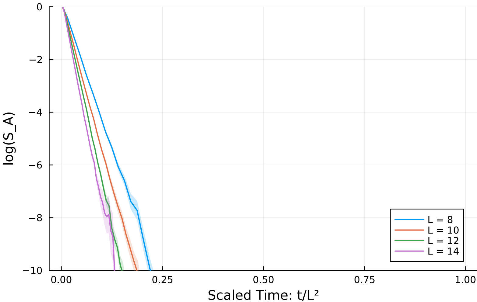
Scaled Log Entropy Evolution ( p = 0.700000 )
